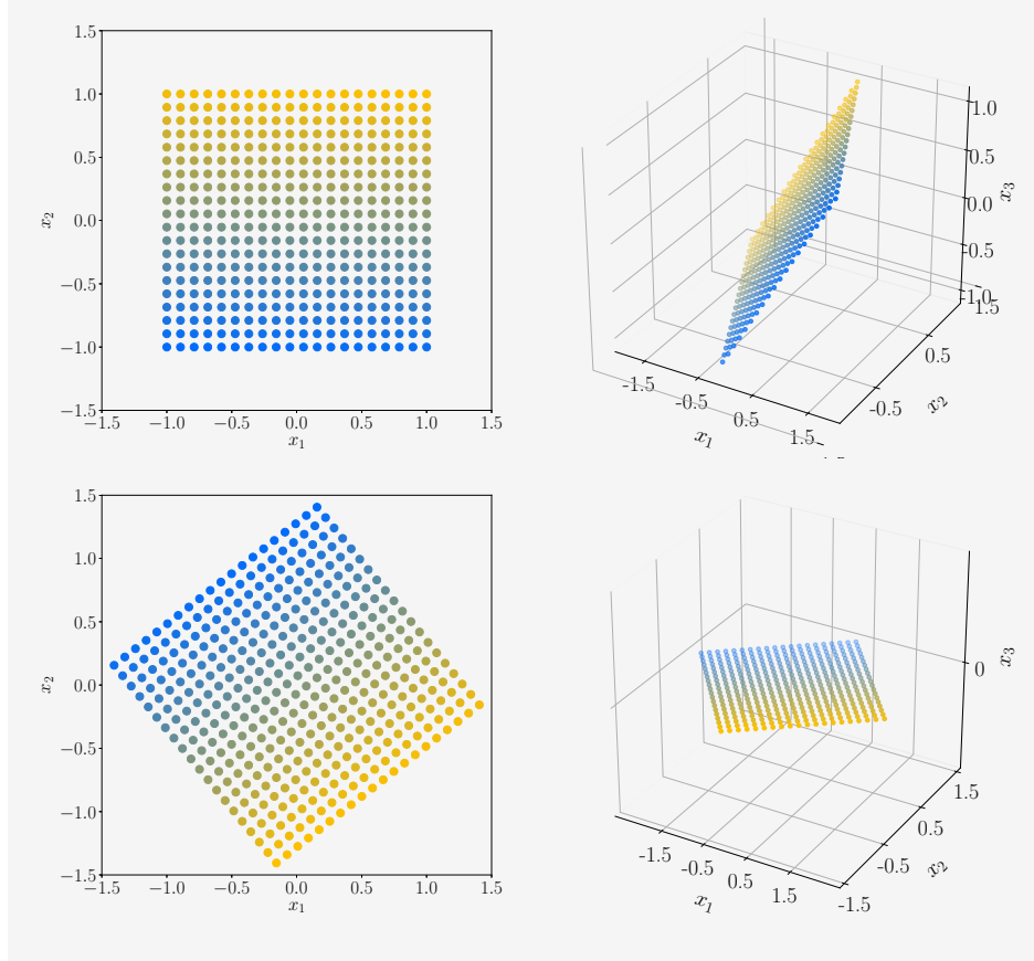
Figure 4.9 SVD and mapping of vectors (represented by discs). The panels follow the same anti-clockwise structure of Figure 4.8.
