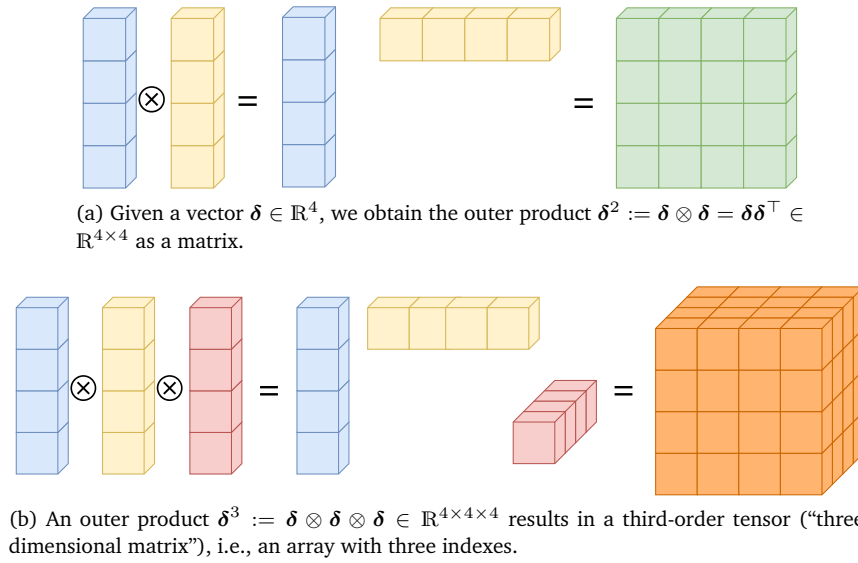
Figure 5.13 Visualizing outer products. Outer products of vectors increase the dimensionality of the array by 1 per term. (a) The outer product of two vectors results in a matrix; (b) the outer product of three vectors yields a third-order tensor.
