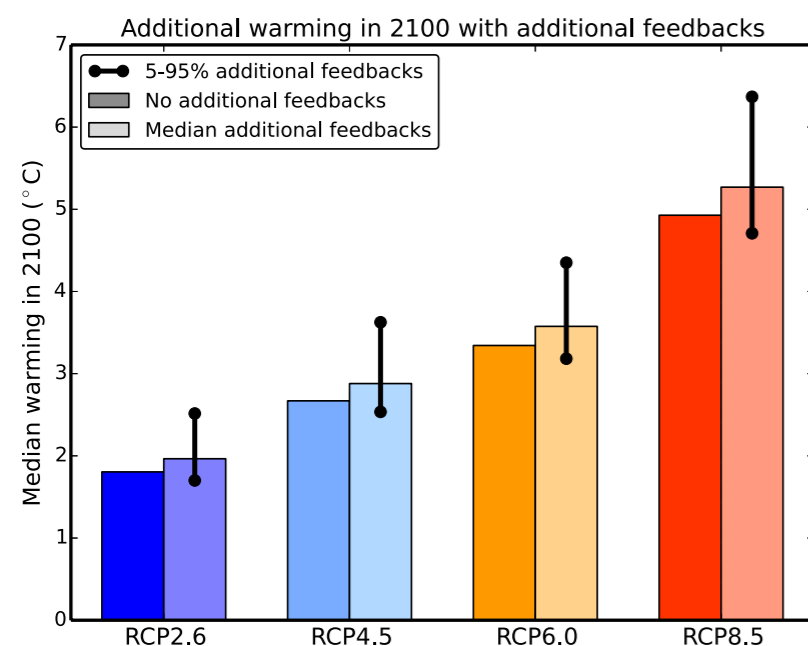
Figure 5: Estimate of added warming from earth system processes considered in the IPCC assessment but not typically included in climate change estimates.
